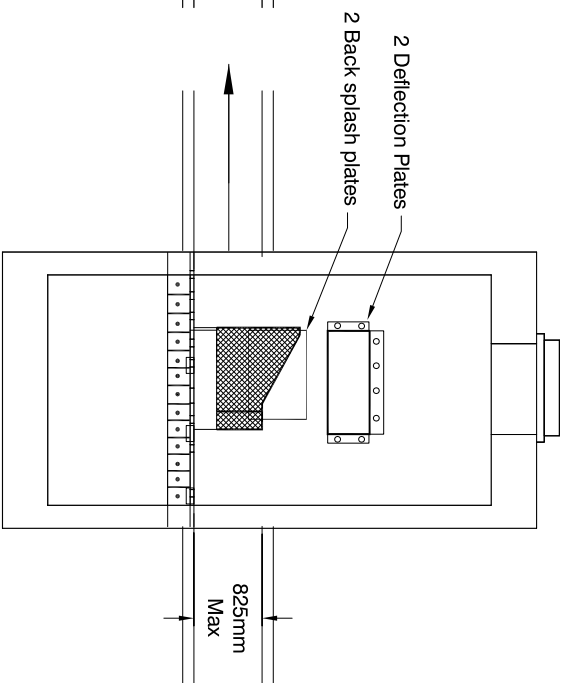
Inlet deflection wall
